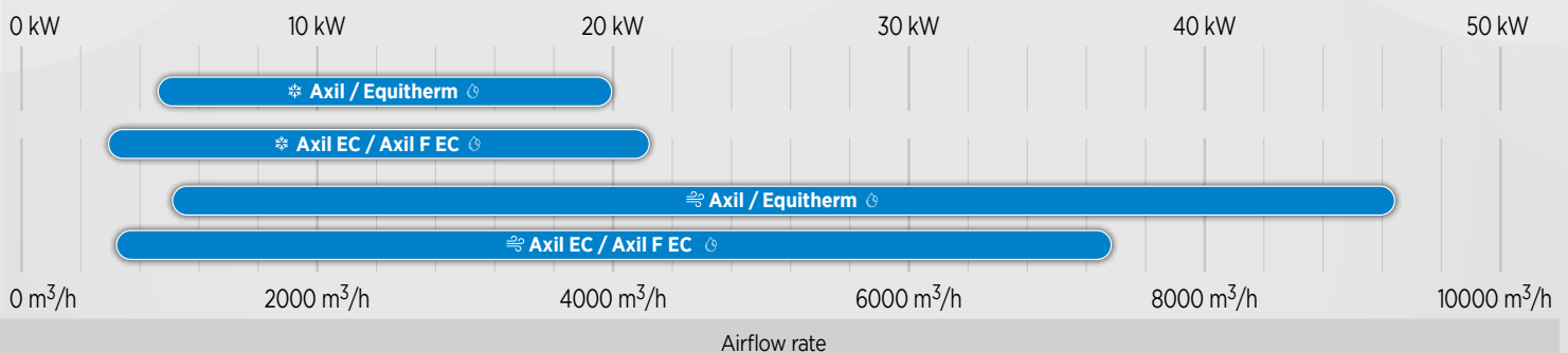
Cooling capacity
